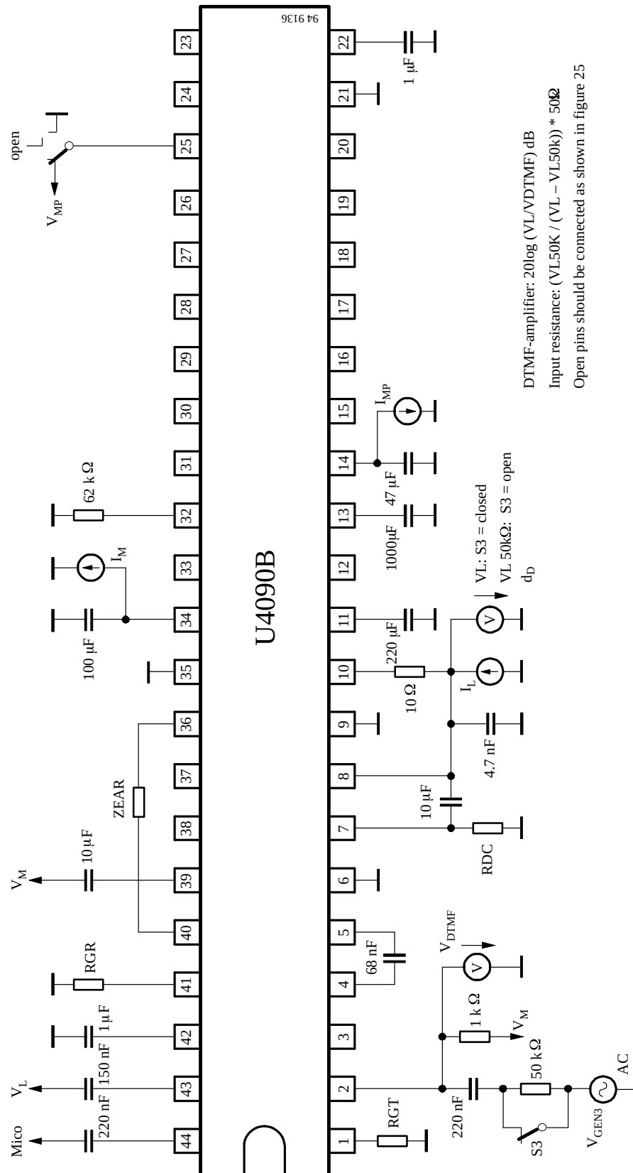
Figure 23. DTMF amplifier
