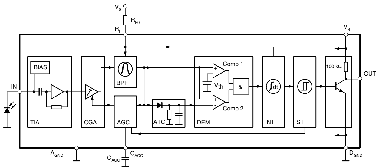
Figure 1-2. Block Diagram
