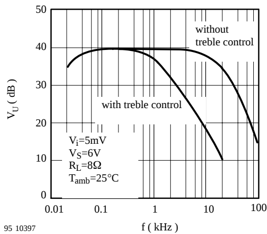
Figure 4. AF section
