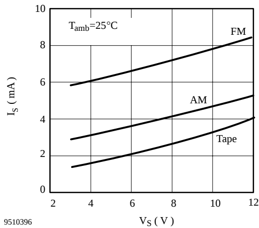
Figure 3. Quiescent current
