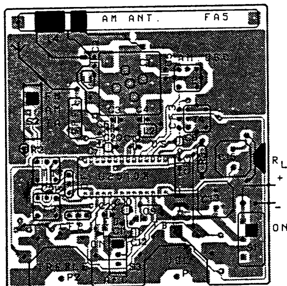
Figure 19. PC-board
