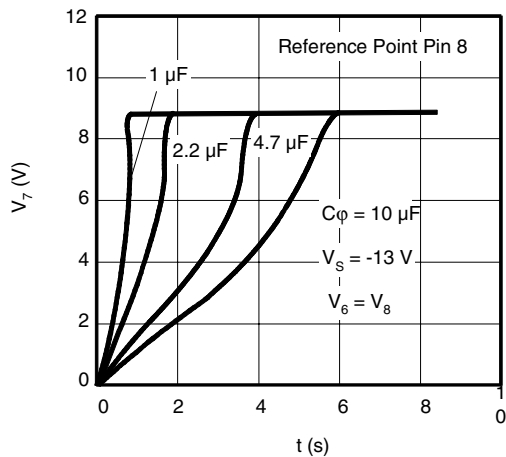
Figure 9. Soft-start Characteristic
