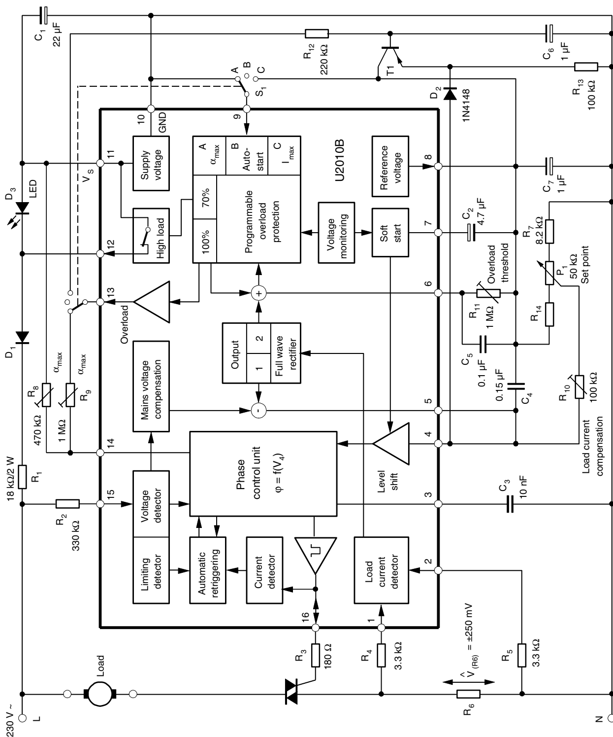
Figure 19. Application Circuit
