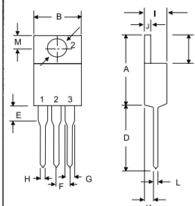
TO-220AB
