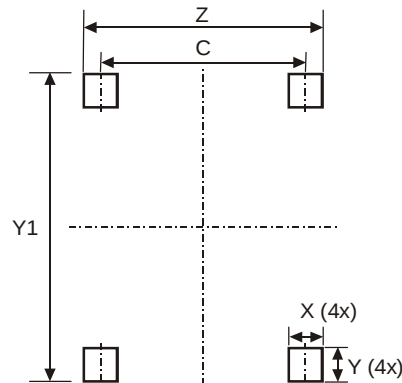
W-DFN5060-4
