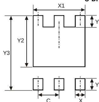
U-DFN2523-6
