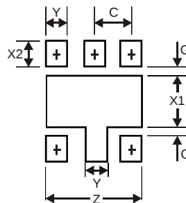
U-DFN2020-6
