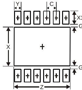
U-DFN3030-12
