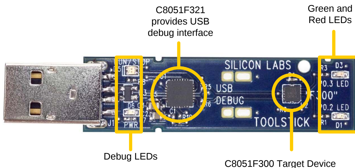
Figure 1. ToolStick Board
