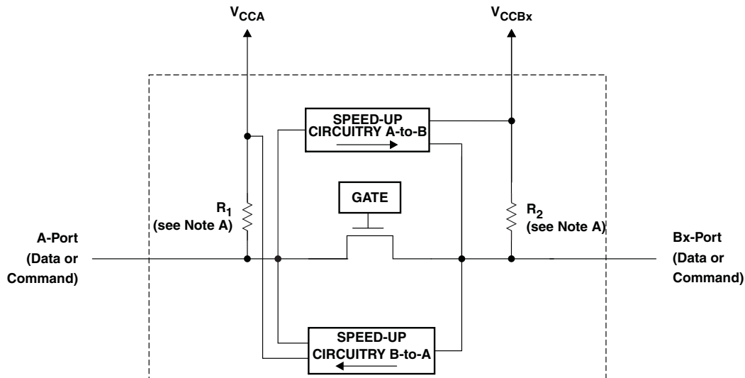
Simplified Architecture of Command and Each Data Path
