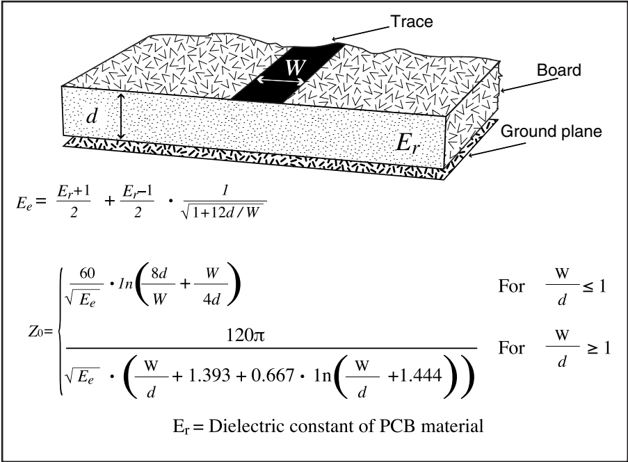
Figure 17: Microstrip Formulas
