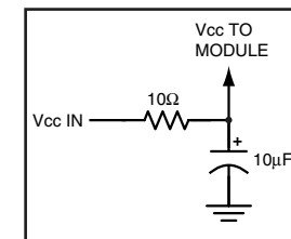
Figure 11: Supply Filter
