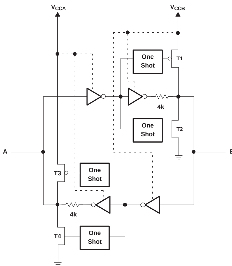
Figure 1. Architecture of TXB0106 I/O Cell
