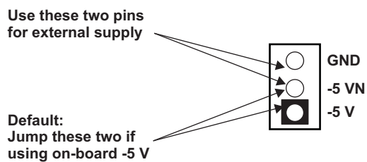
Figure 10. Jumper J54
