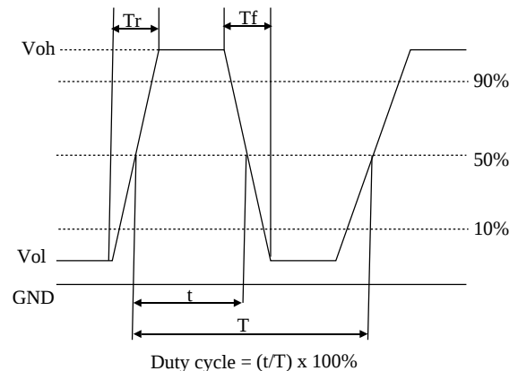
Test waveform
