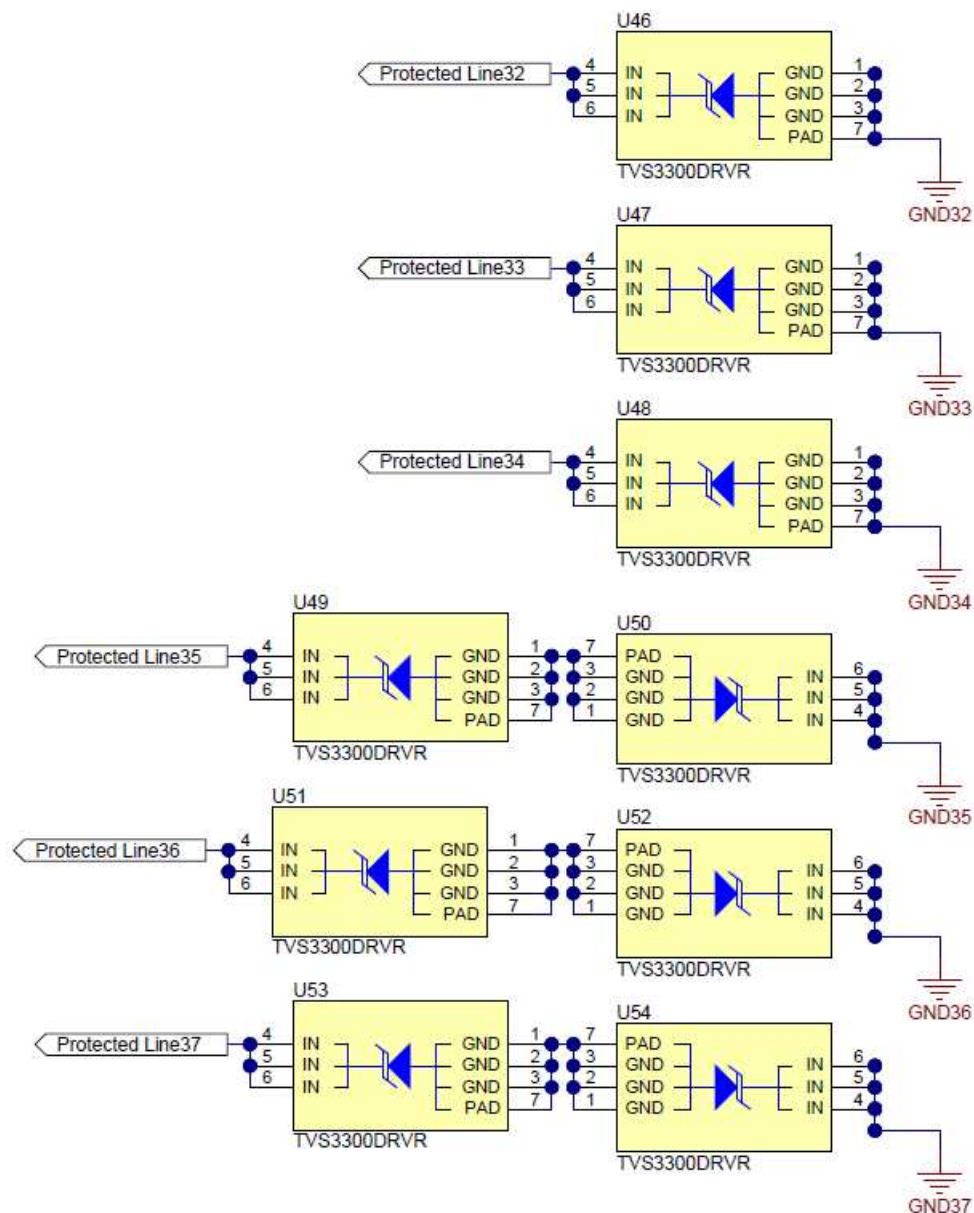
Figure 9. TVS3300 Schematic
