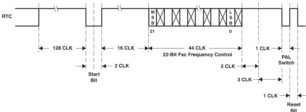
Figure 3-7. RTC Timing
