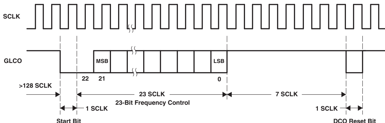
Figure 3-6. GLCO Timing
