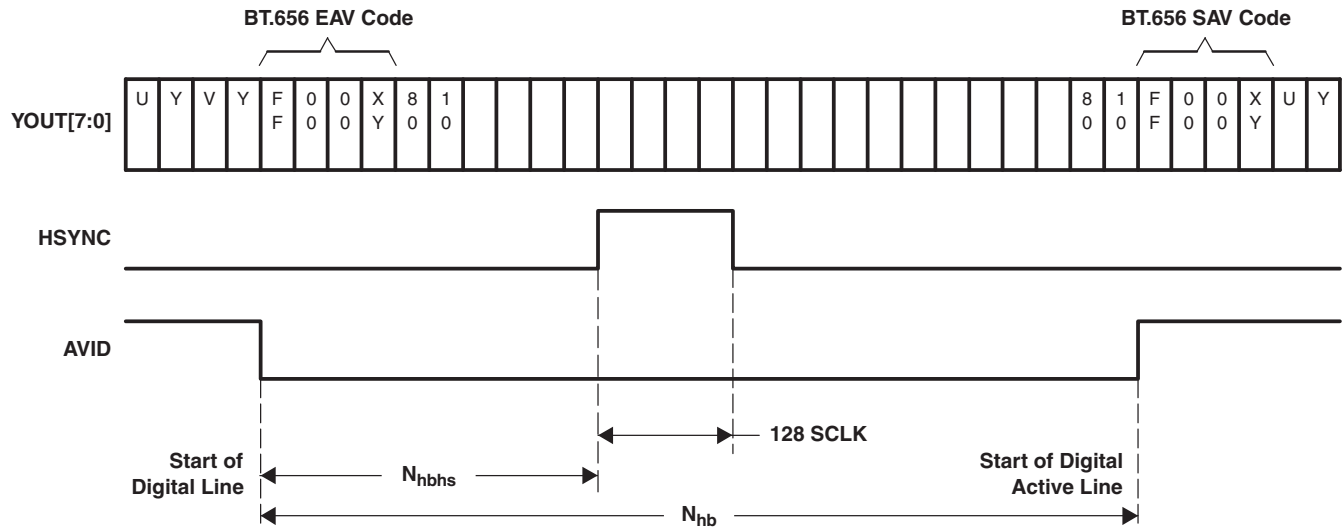
Figure 3-9. Horizontal Sync
