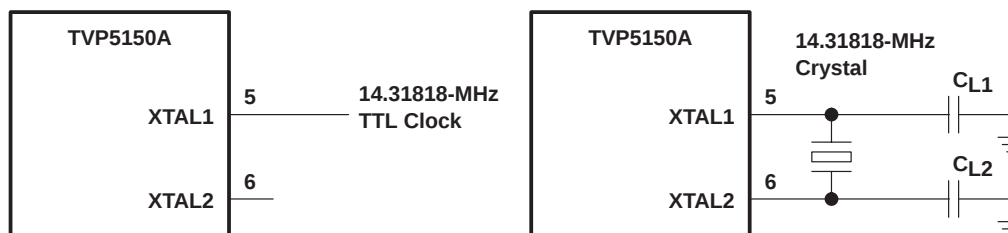
Figure 2–5. Reference Clock Configurations
