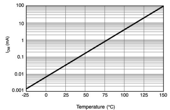
Figure SB6 - Off-state Current vs. Temperature
