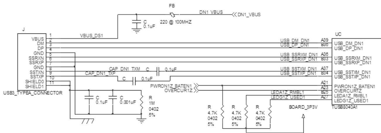
Figure 6-5. Downstream Port 3 Implementation
