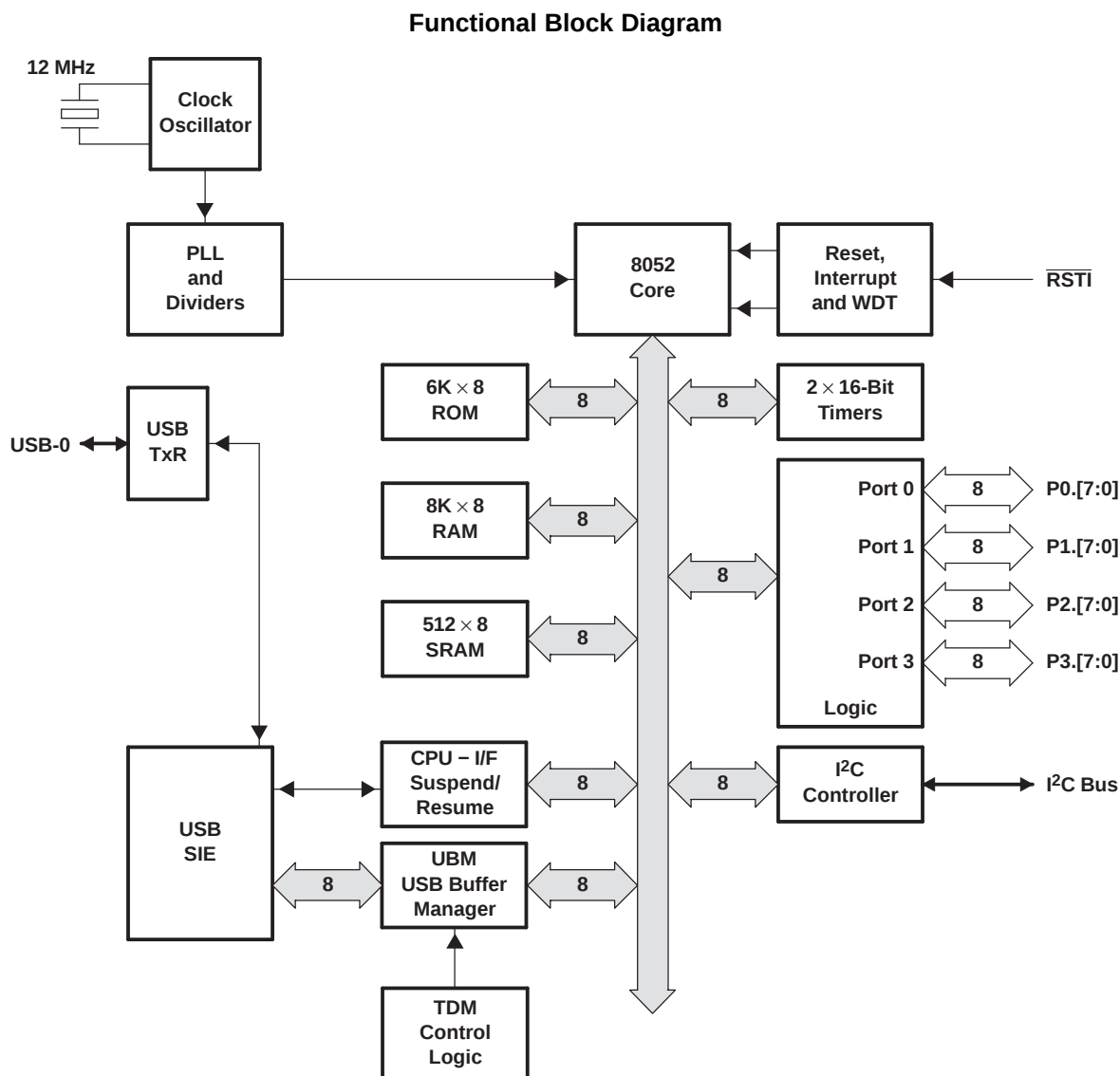
Figure 1-1. TUSB3210 Block Diagram
