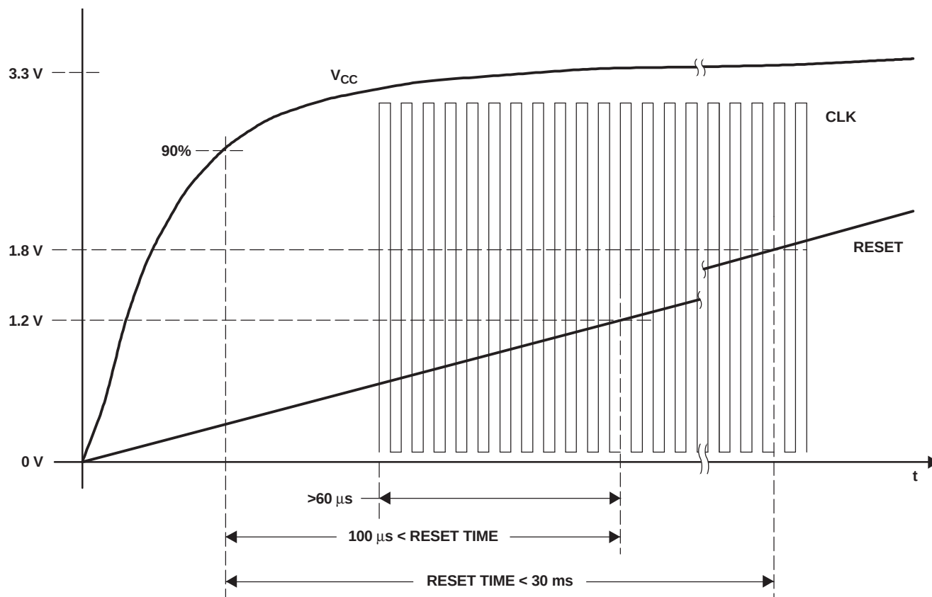
Figure 4-4. Reset Timing
