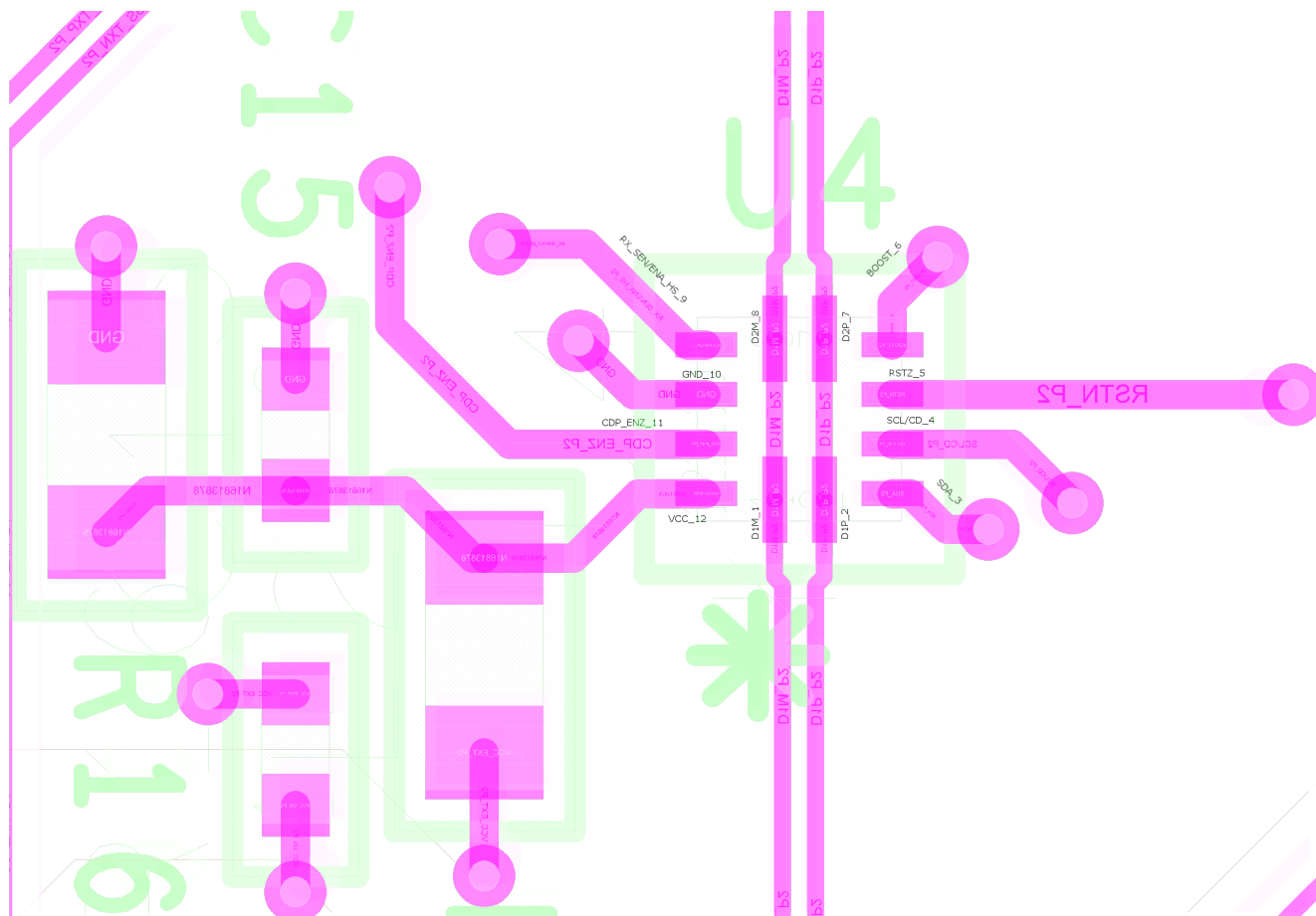
Figure 11-1. Layout Example
