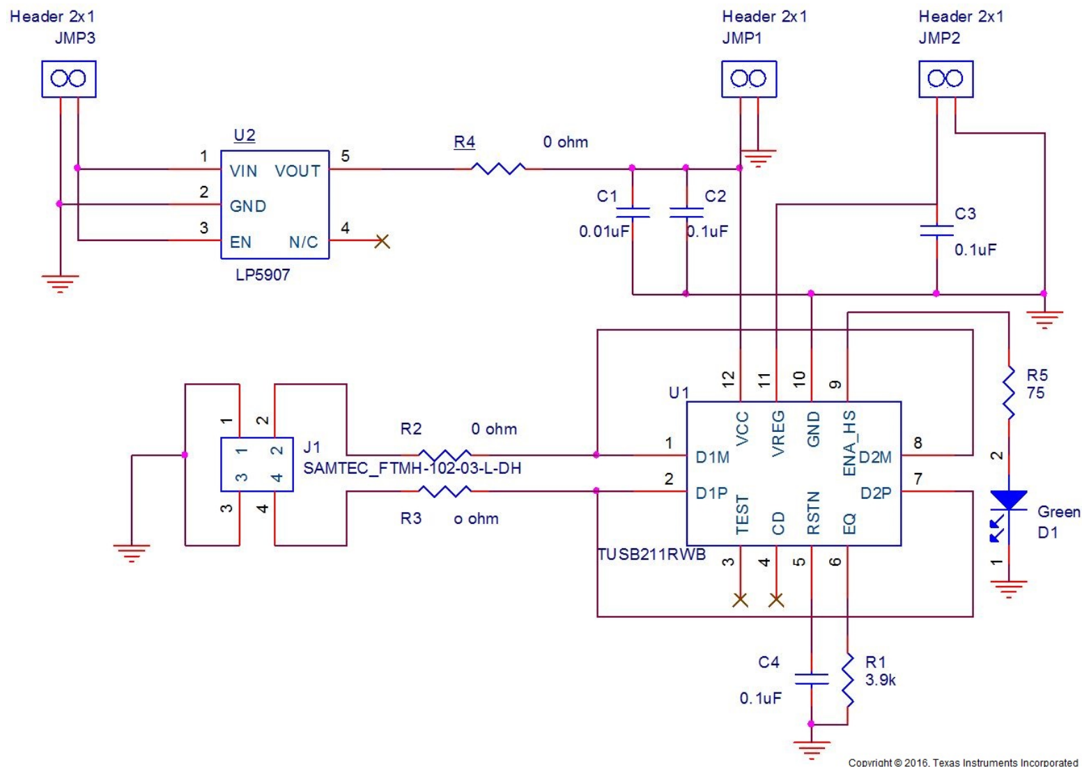
Figure 2. TUSB211 EVM Schematics
