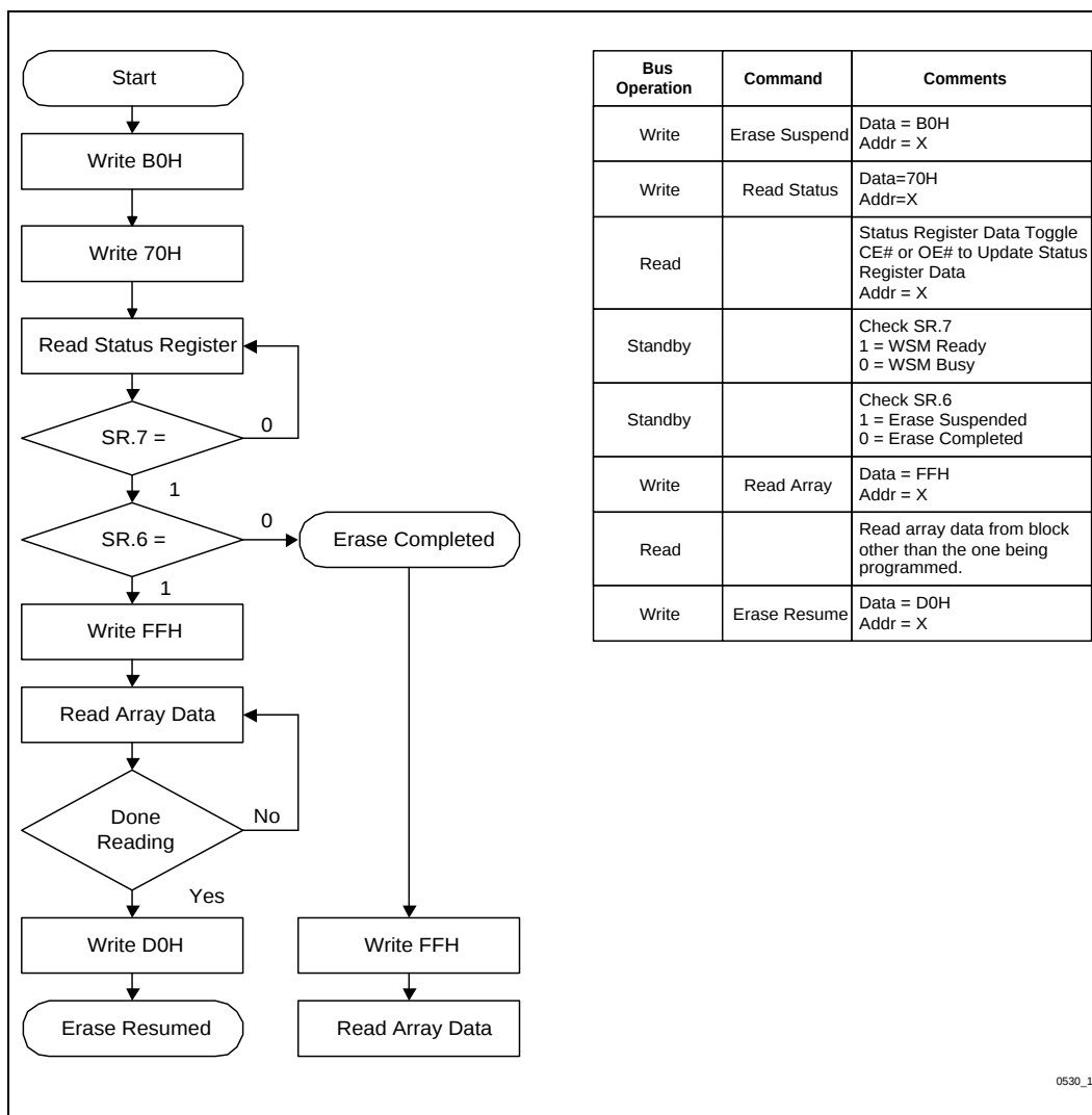
Figure 11. Erase Suspend/Resume Flowchart
