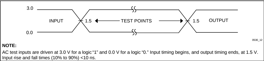
Figure 19. 3.3 V Input Range and Measurement Points
