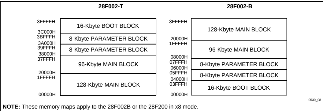
Figure 8. Byte-Wide x8-Mode Memory Maps
