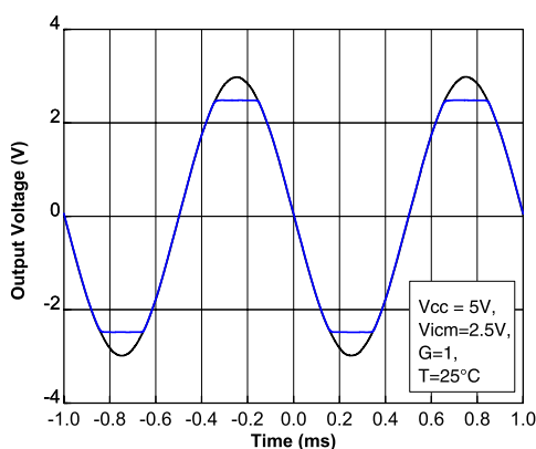
Figure 60. No phase reversal
