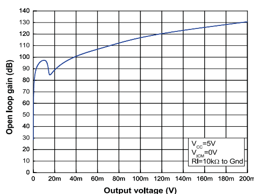
Figure 61. Gain vs. output voltage, V_{CC} = 5\text{ V} , R_I = 10\text{ k}\Omega to GND
