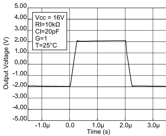
Figure 26: Large step response
