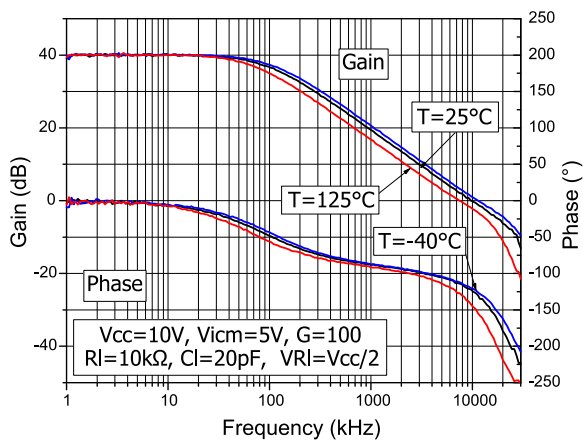
Figure 16: Bode diagram vs. temperature for V_{CC} = 10V
