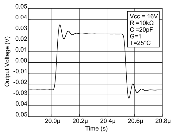
Figure 27: Small step response
