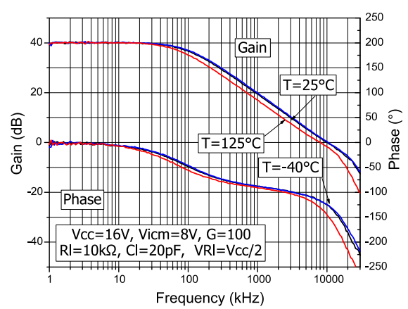
Figure 17: Bode diagram vs. temperature for V_{CC} = 16V
