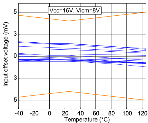
Figure 6: Input offset voltage vs. temperature at VCC = 16 V
