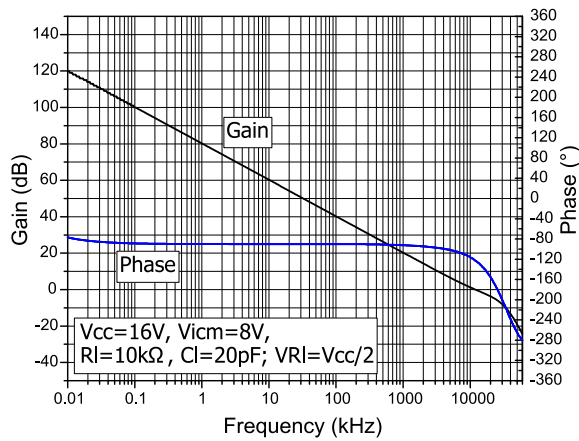
Figure 14: Open loop gain vs. frequency
