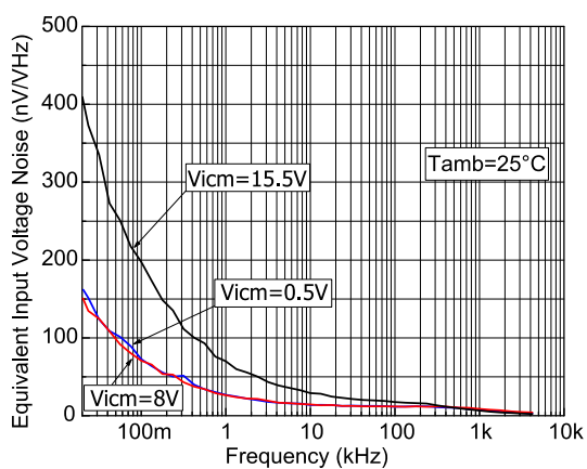
Figure 30: Noise vs. frequency with 16 V supply voltage
