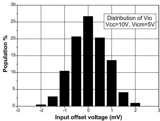
Figure 4: Distribution of input offset voltage at VCC = 10 V
