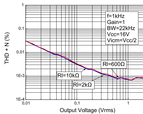
Figure 33: THD+N vs. output voltage at V_{CC} = 16\text{ V}
