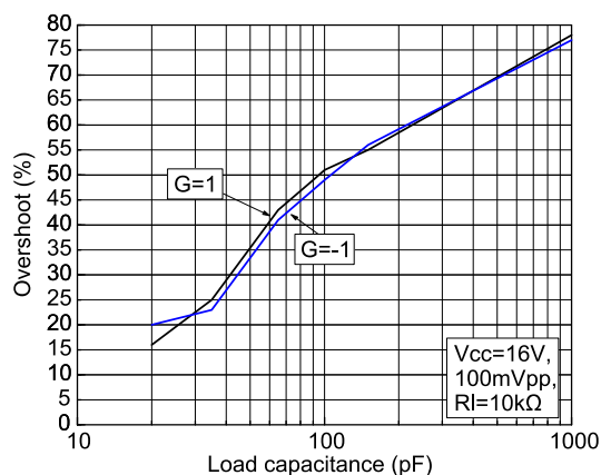
Figure 24: Overshoot vs. capacitive load without feedback capacitor
