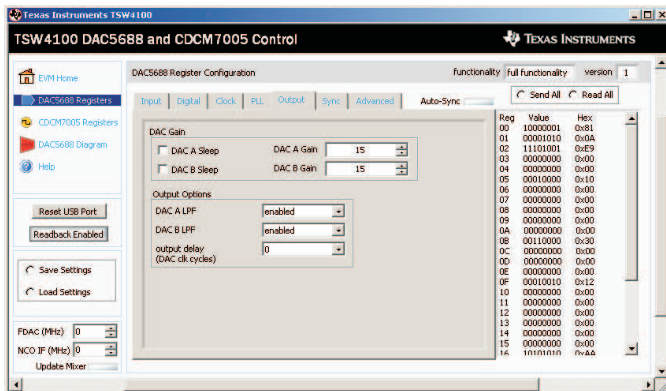
Figure 20. DAC Gain
