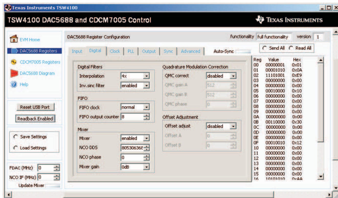
Figure 18. DAC5688 Filters
