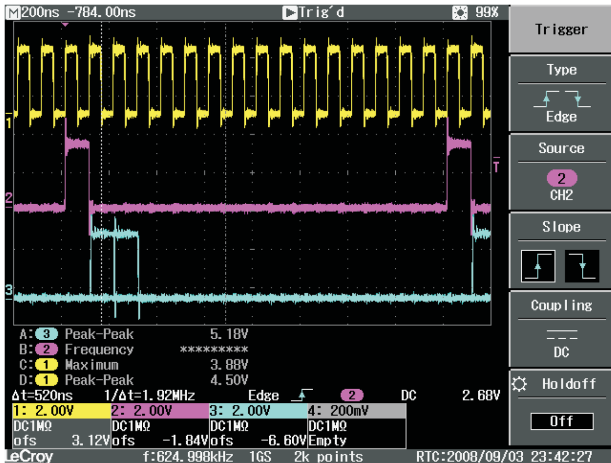
Figure 58. Channel 1 Interface Timing With a Sync Delay of 96 and Negative SCK Polarity
