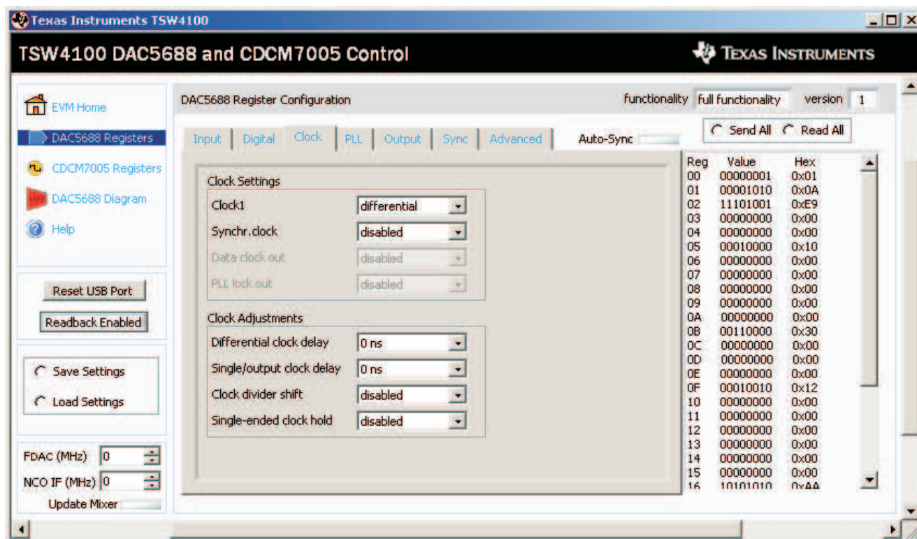
Figure 19. Clock Settings
