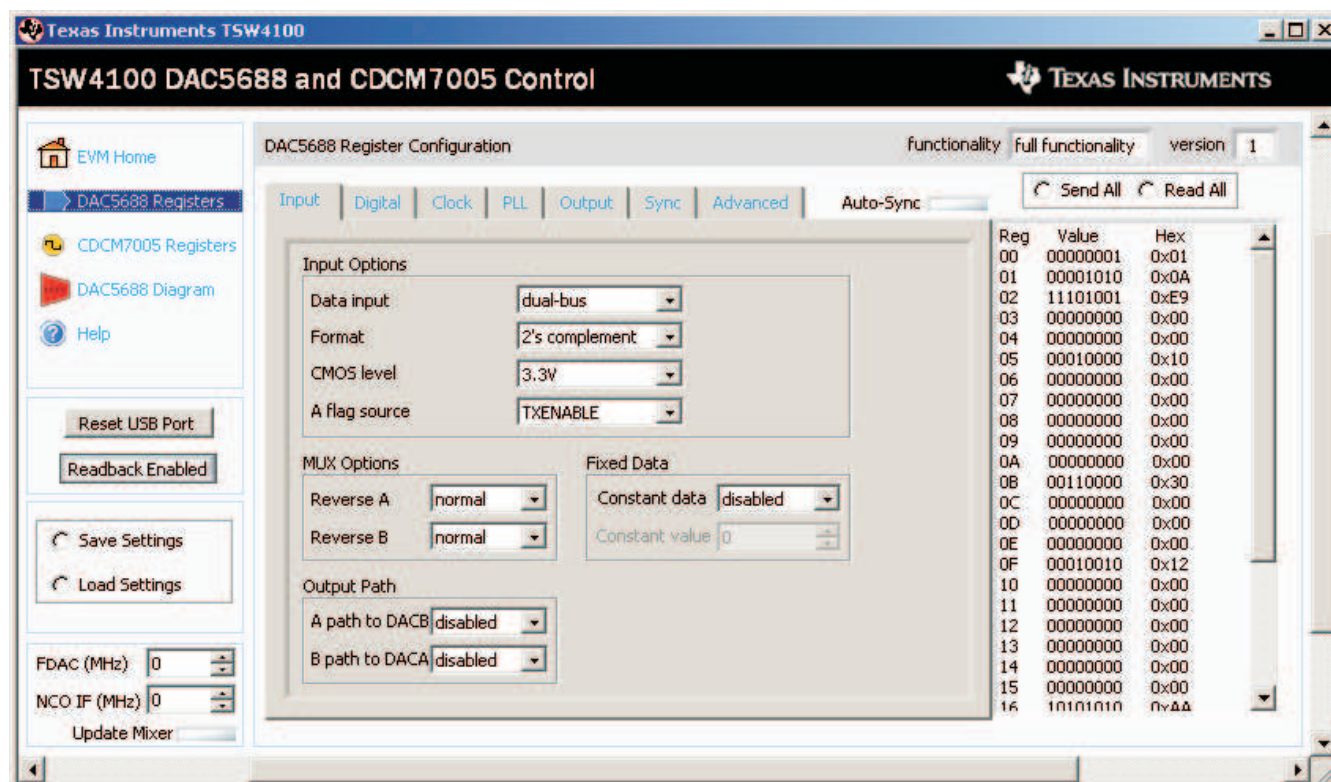
Figure 17. DAC5688 Options
