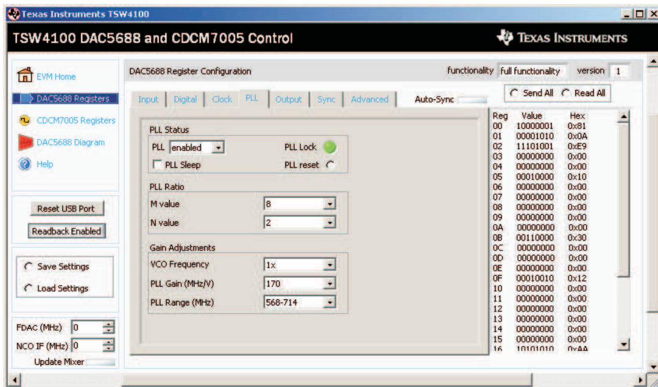
Figure 16. DAC5688 Interface
