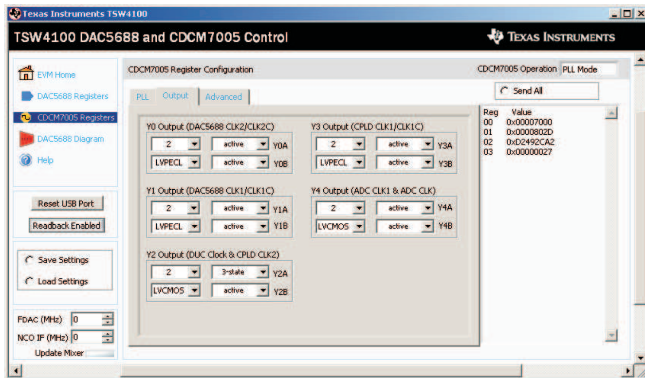
Figure 15. CDCM7005 Interface
