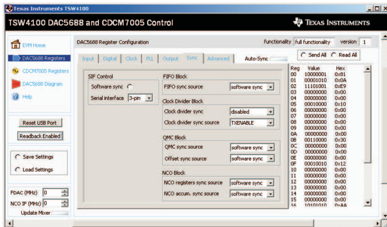
Figure 21. SIF Control
