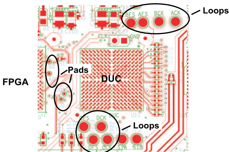
Figure 55. Test Points
