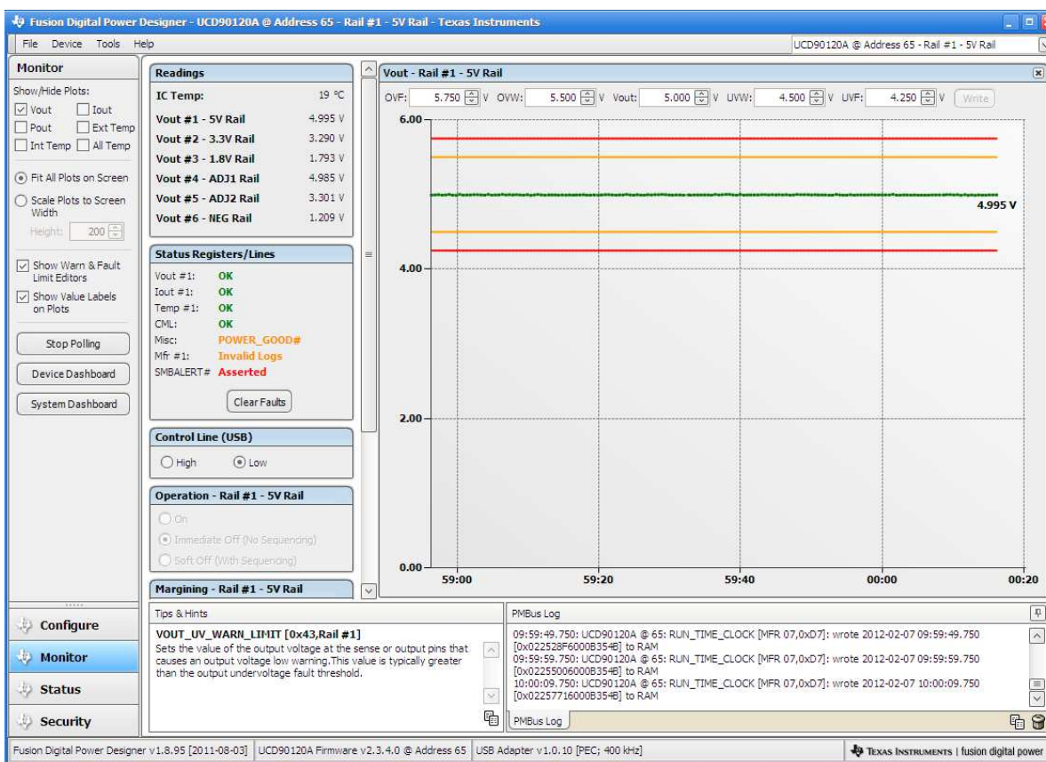
Figure 5. Voltage Monitoring Readouts For Each Output Voltage Rail
