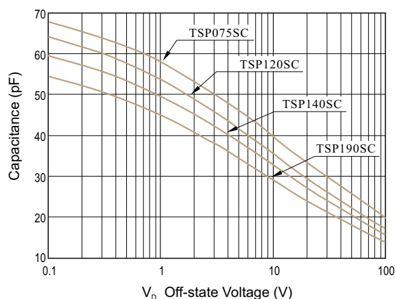
TYPICAL CAPACITANCE V.S. OFF-STATE VOLTAGE
