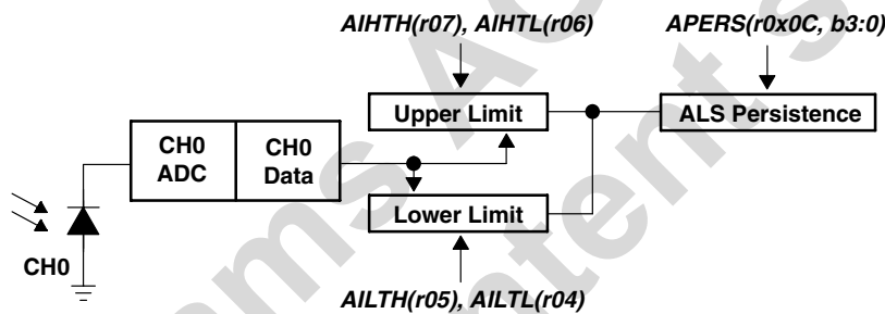
Figure 8. Programmable Interrupt
