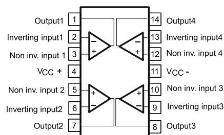
Pin connections TSH84 TSSOP14
