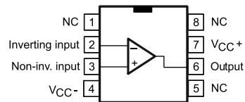
Pin connections TSH80/SO8
