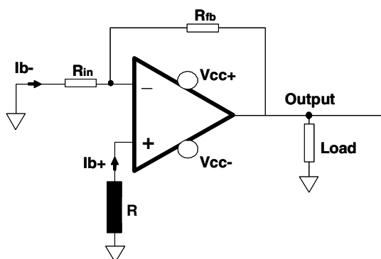
Figure 30: Compensation of the input bias current
