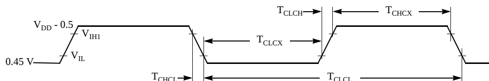
Figure 25. External Clock Waveform
