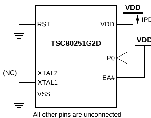
Figure 32. I_{PD} Test Condition, Power-Down Mode
