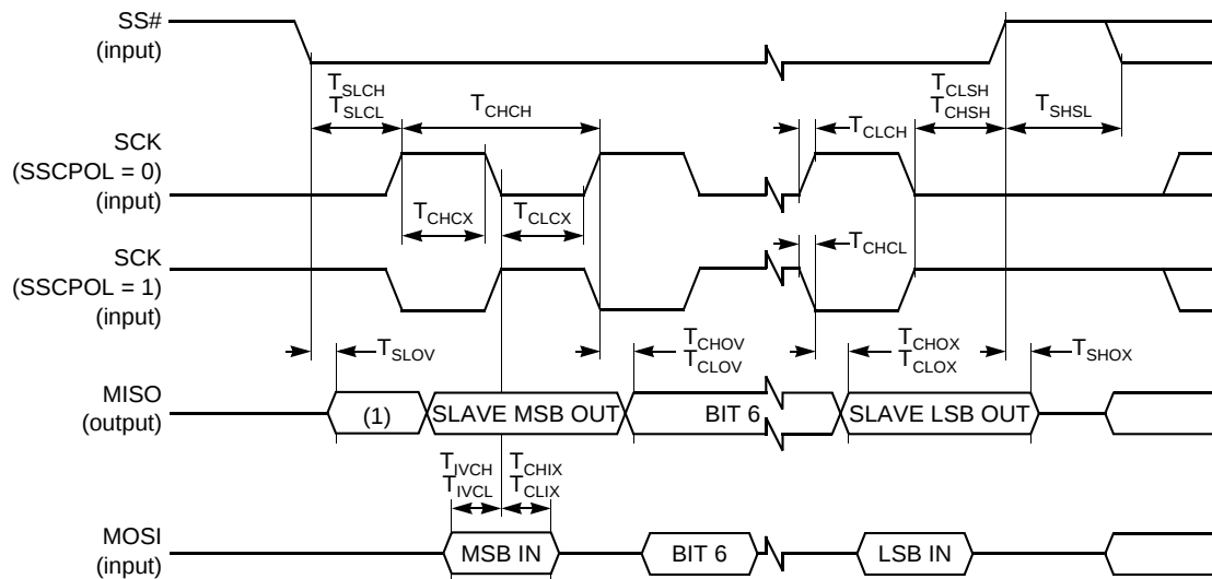
Figure 22. SPI Slave Waveforms (SSCPHA = 1)
