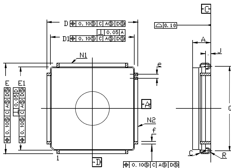
Figure 36. Ceramic Quad Pack J
