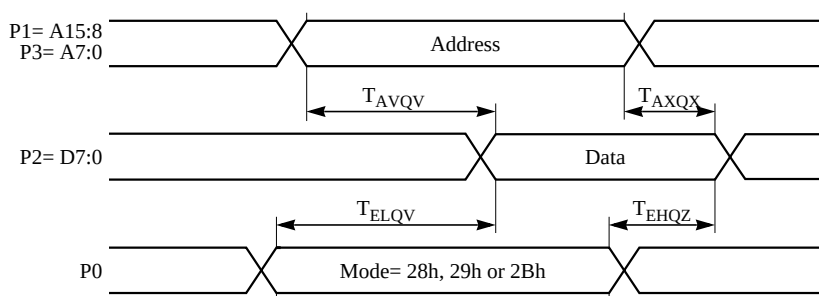
Figure 32. EPROM Verifying Waveforms
