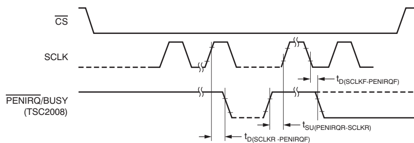
Figure 2. PENIRQ Timing
