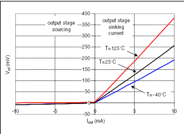
Figure 7. Output stage low-state saturation voltage versus output current ( V_{\text{sense}} = -1 \text{ V} )
