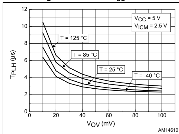
Figure 26. Propagation delay T_{PLH} vs. input signal overdrive at V_{CC} = 5\text{ V}
