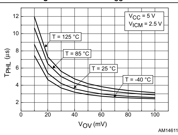
Figure 27. Propagation delay T_{PHL} vs. input signal overdrive at V_{CC} = 5\text{ V}
