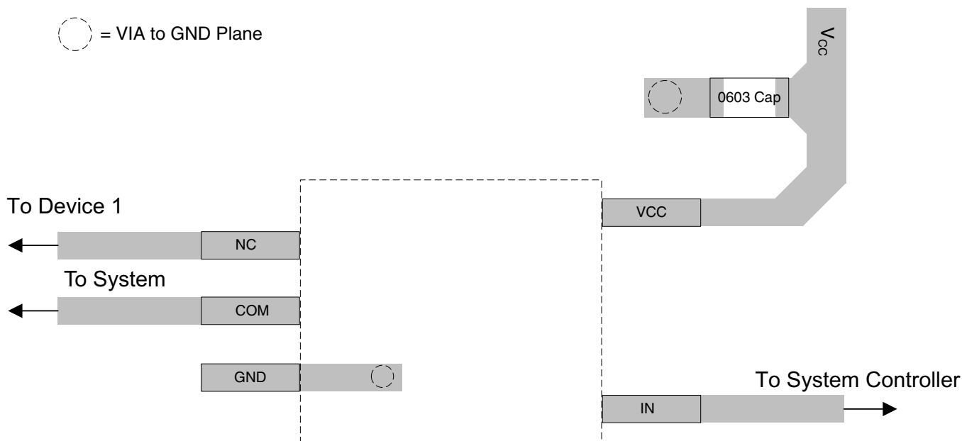
Figure 24. Example Layout
