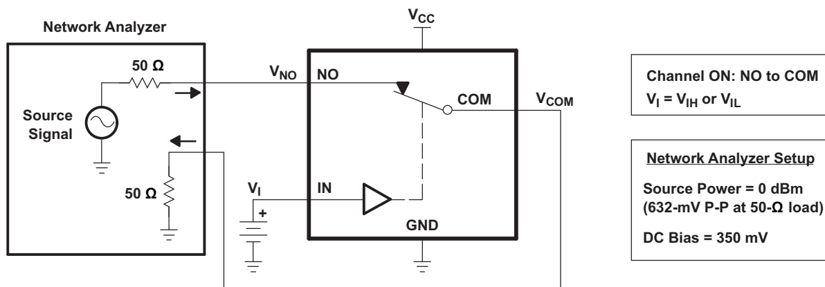
Figure 19. Turnon ( t_{ON} ) and Turnoff Time ( t_{OFF} )
