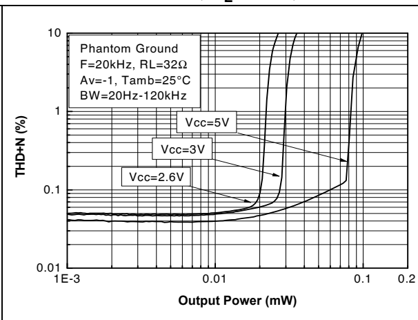
Figure 11. THD+N vs. output power, PHG, F = 20 kHz, R_L = 32\ \Omega , A_v = 1
