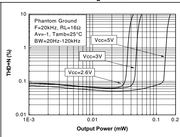
Figure 9. THD+N vs. output power, PHG, F = 20 kHz, R_L = 16\ \Omega , A_v = 1
