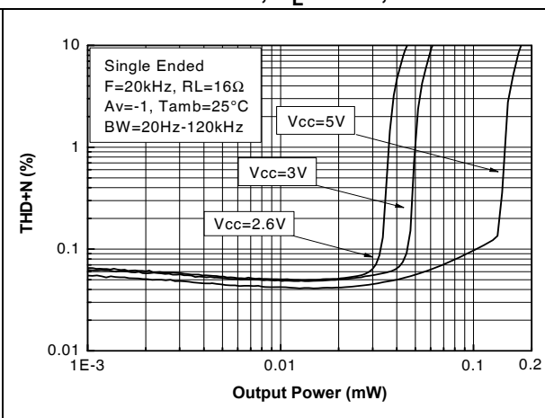
Figure 13. THD+N vs. output power, SE, F = 20 kHz, R_L = 16\ \Omega , A_v = 1
