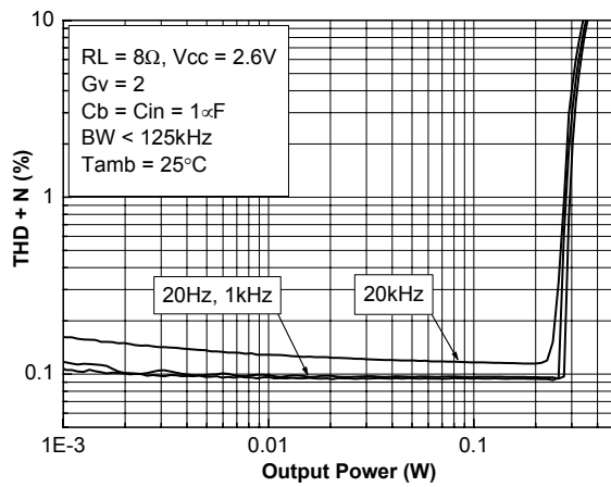
Figure 32. THD + N vs output power R_L = 8\ \Omega , V_{CC} = 2.6\text{V}
