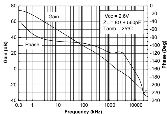
Figure 7. Open loop frequency response V_{CC}=2.6\text{ V} , Z_L=8\Omega
