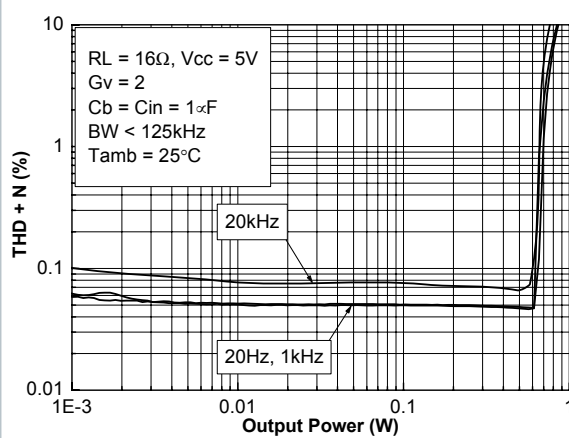
Figure 40. THD + N vs output power RL=16\text{ }\Omega V_{cc}=5\text{ V}
