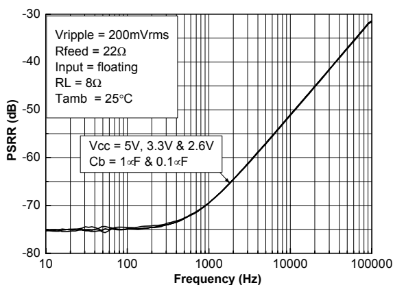
Figure 11. Power supply rejection ratio (PSRR) vs power supply
