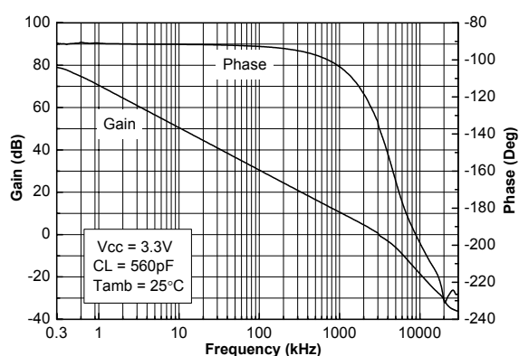
Figure 9. Open loop frequency response V_{CC}=3.3\text{ V} , C_L=560\text{ pF}
