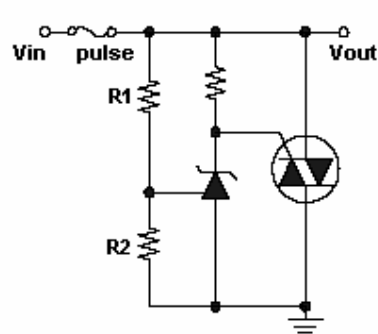
Figure 9. Crow Bar
