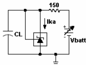
test circuit for curve A
