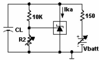
test circuit for curve B, C, D
