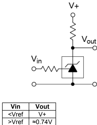
Figure 9. Single-Supply Comparator with Temperature-Compensated Threshold
