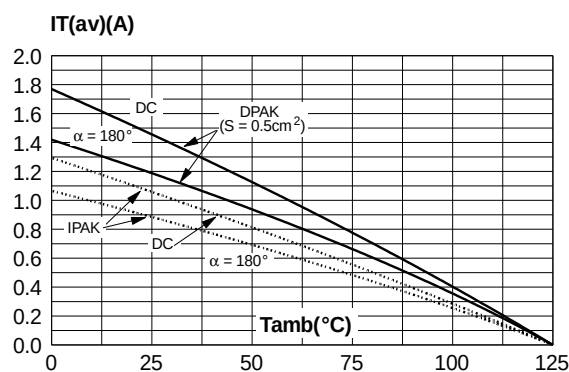
Fig. 2-2: Average and D.C. on-state current versus ambient temperature (device mounted on FR4 with recommended pad layout) (DPAK).
