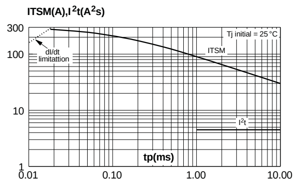
Fig. 9: Non-repetitive surge peak on-state current for a sinusoidal pulse with width t_p < 10\text{ms} , and corresponding values of I^2t .
