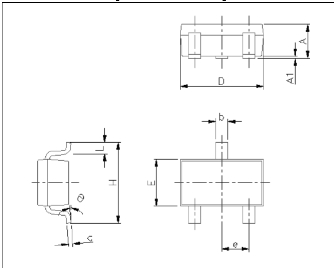
Figure 13. SOT323-3L drawings
