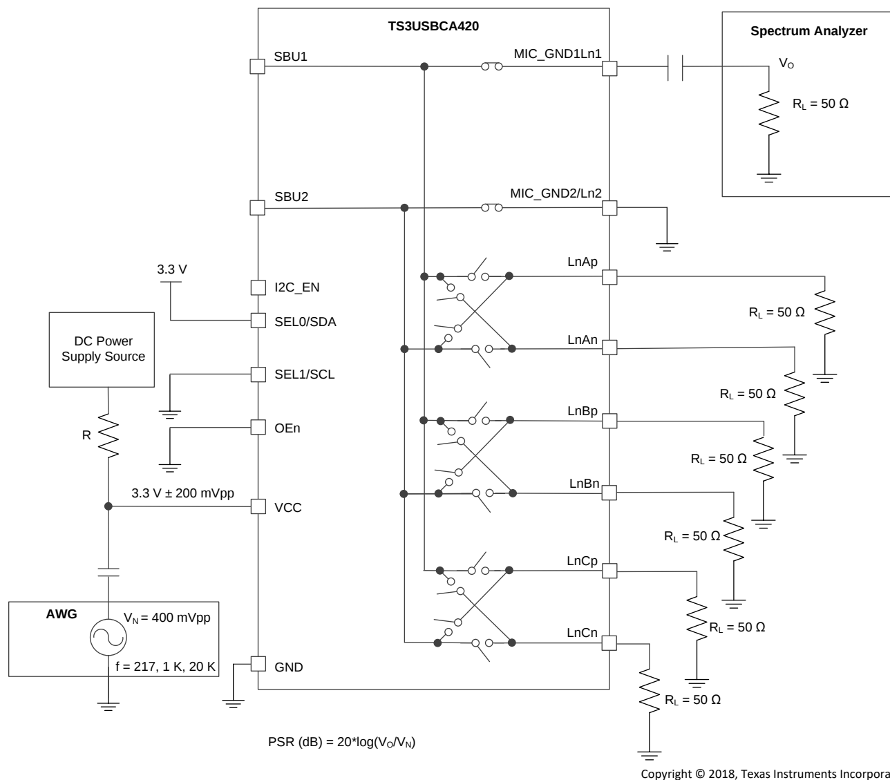
Figure 10. Power Supply Rejection (PSR)
