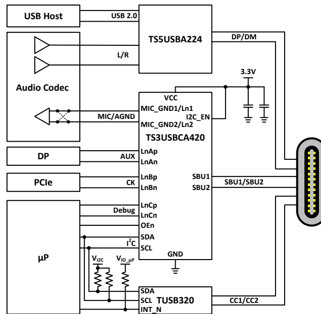
Figure 21. Application of TS3USBCA420 in I 2 C-Configuration Mode
