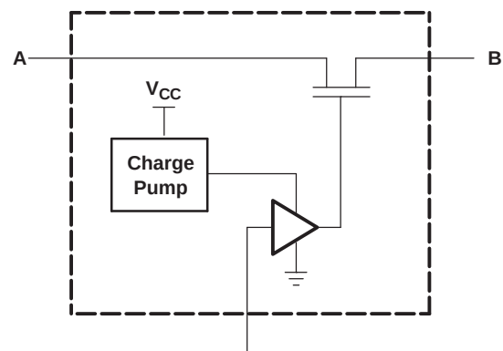
Simplified Schematic, Each FET Switch (SW)
