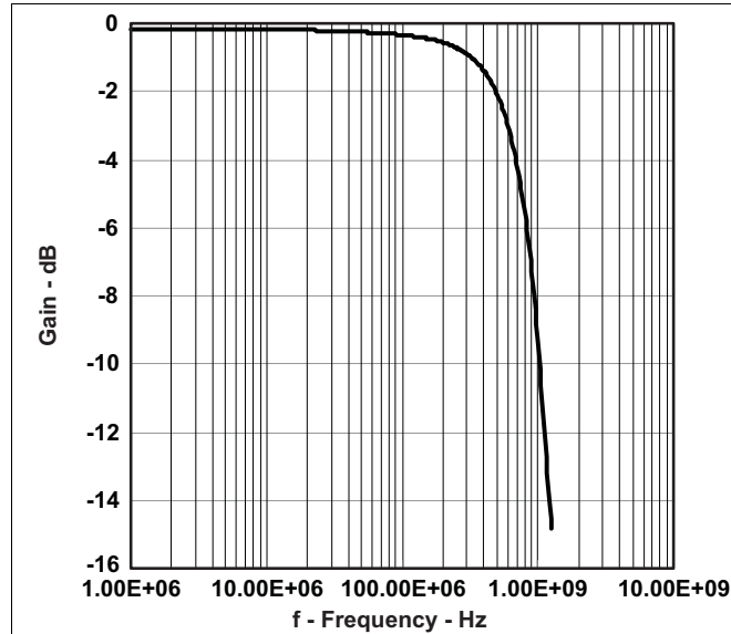
Figure 1. Gain vs Frequency
