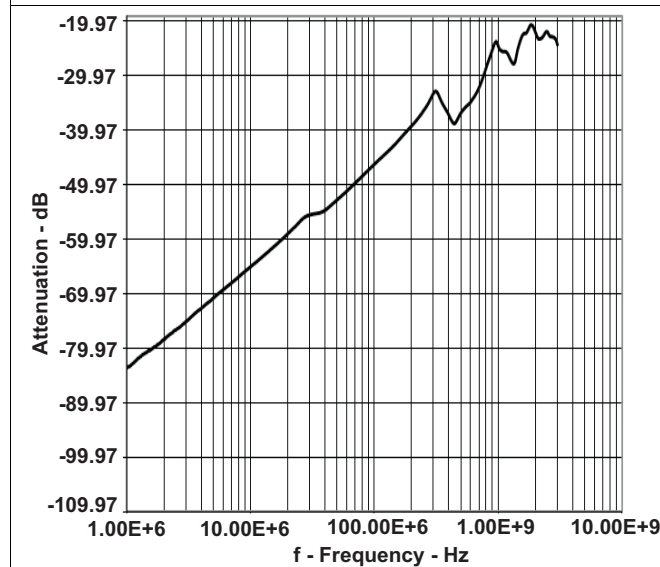
Figure 3. Crosstalk vs Frequency
