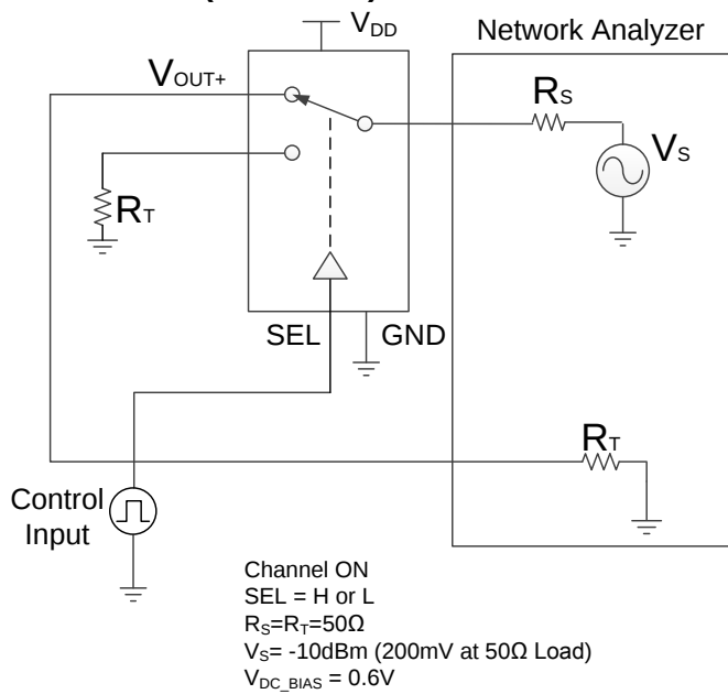
Figure 17. Bandwidth Measurement
