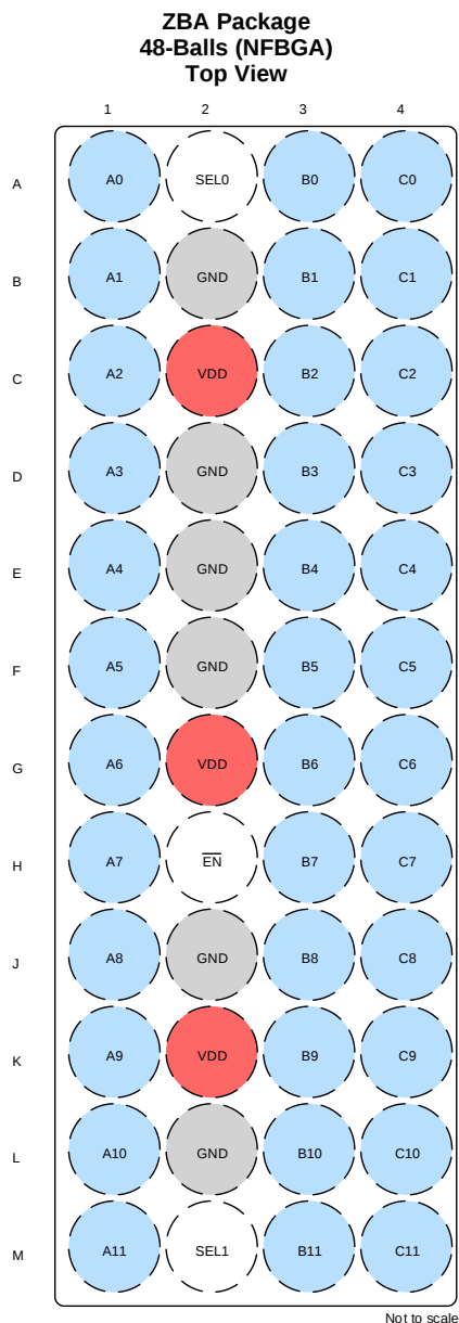
Pin Functions
