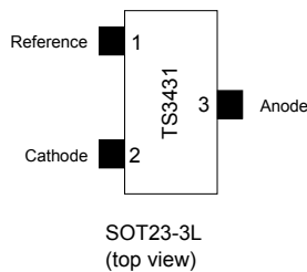
SOT23-3L (Plastic micropackage)
