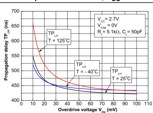
Figure 19. Propagation delay versus overdrive with positive transition, V_{CC} = 2.7 V
