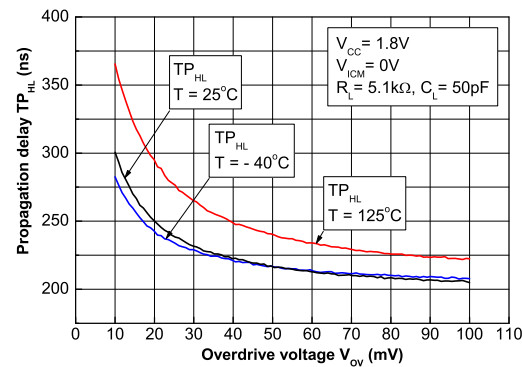
Figure 15. Propagation delay versus overdrive with negative transition, V_{CC} = 1.8 V
