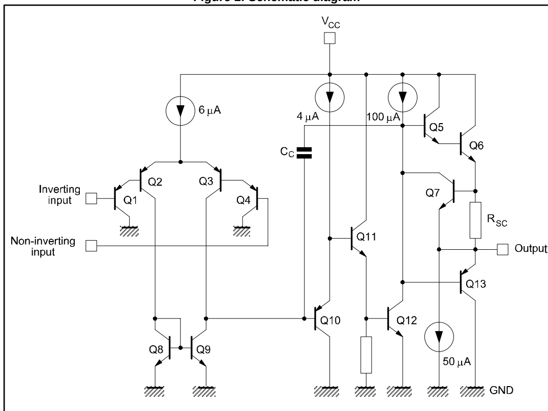
Figure 1: Schematic diagram
