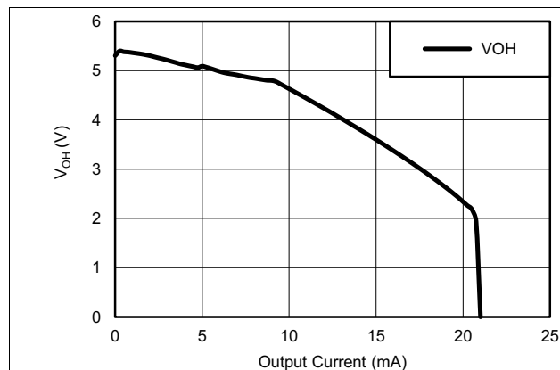
Figure 1. DOUT V_{OH} vs Load Current, Both Drivers Loaded
